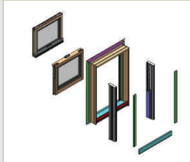
Exploded View
