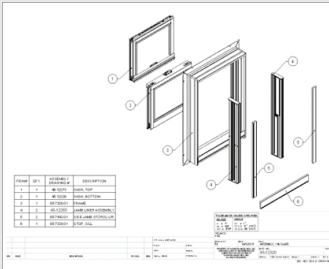
Assembly Drawing
